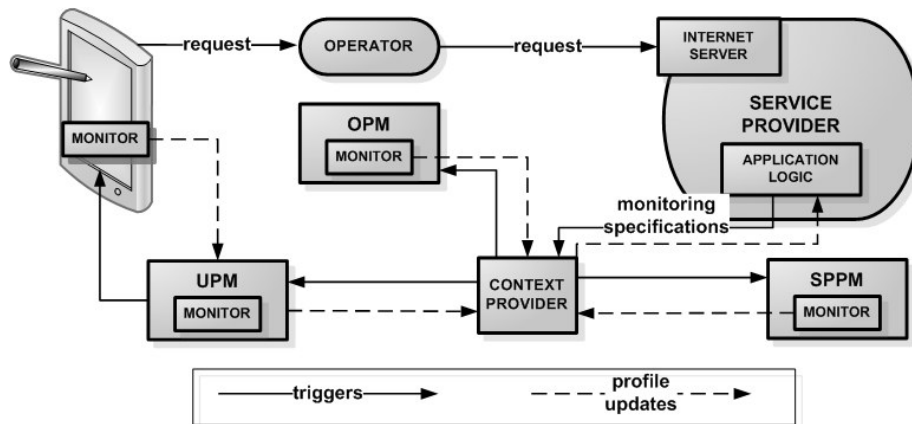
Figure 2. Trigger mechanism
